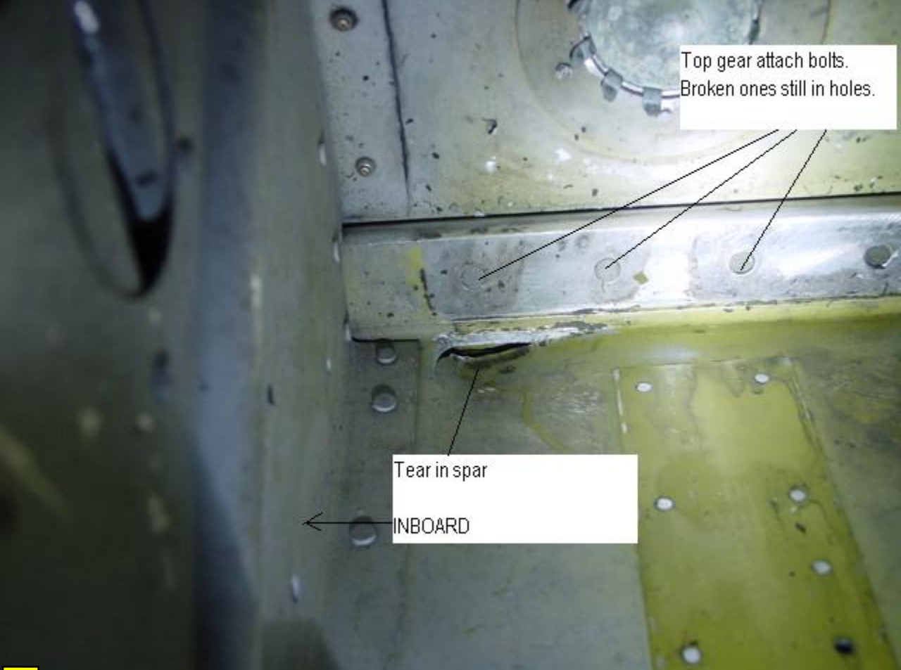
Photograph #2: Interior View of Right Wing (Courtesy of FAA)
