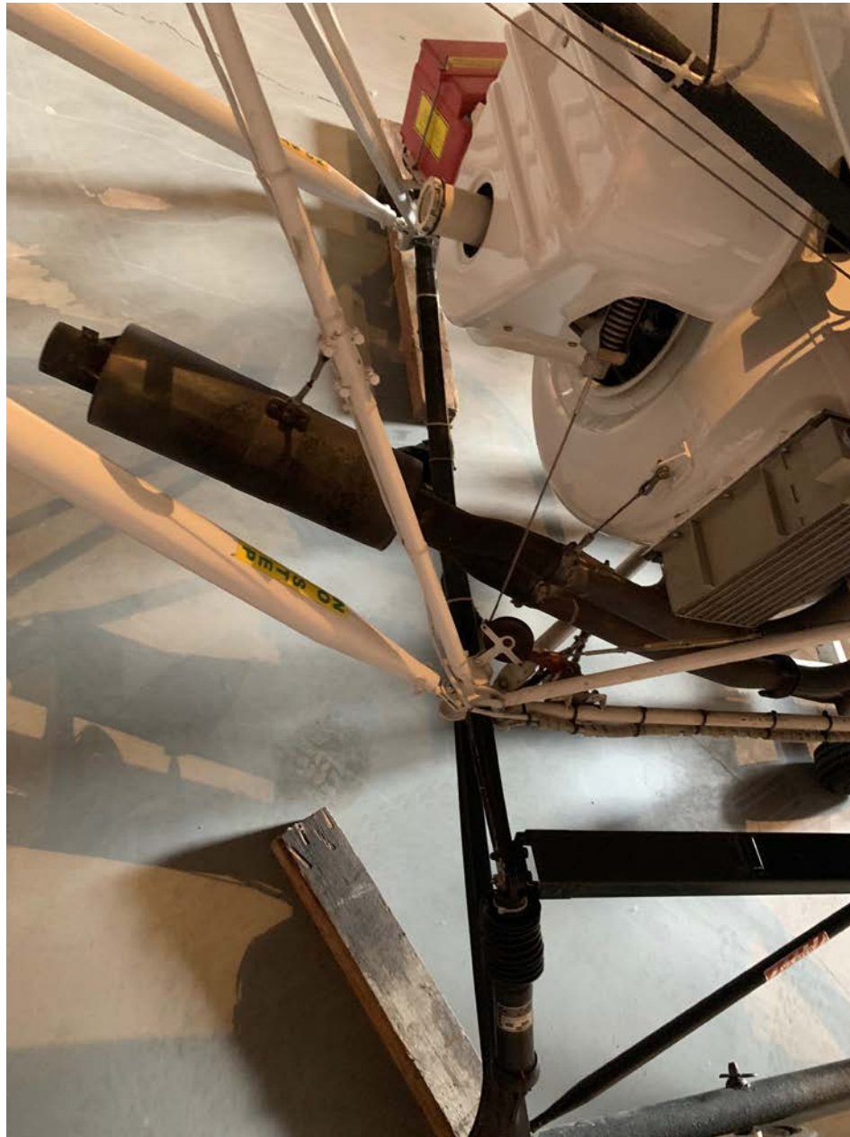
Photo 1 – View of damage to the aft horizontal crossmember (Courtesy of Operator)
