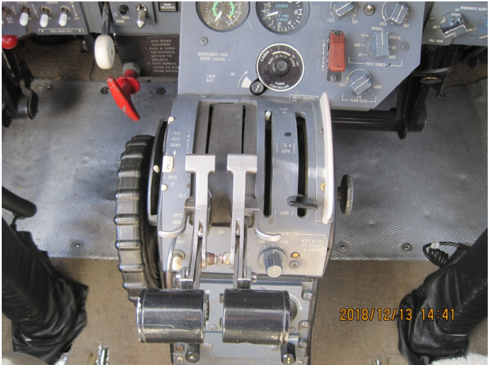
Photo 14 – View of the airplane’s center pedestal (FAA photo)
