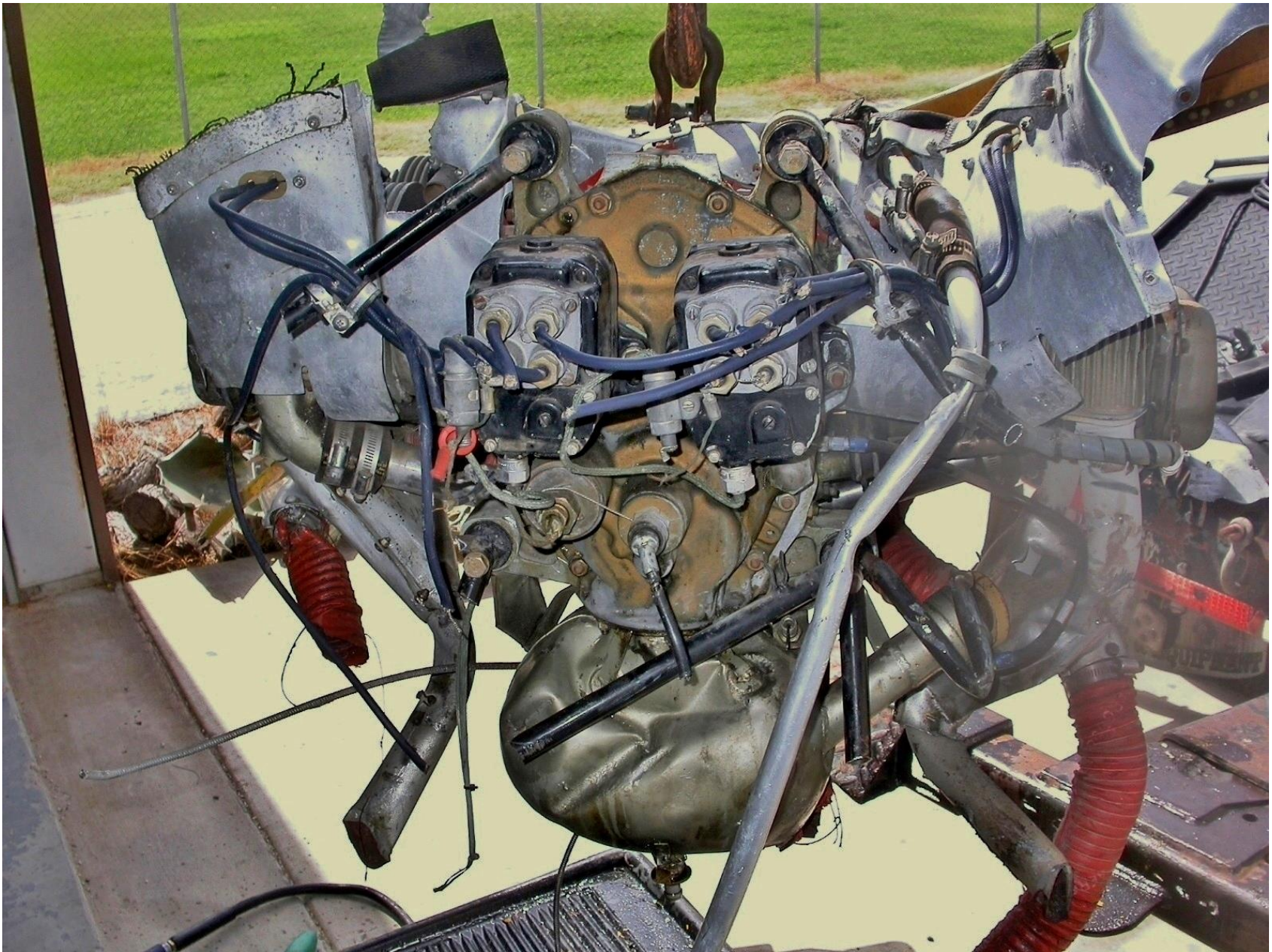
Photo 8 – View of the back of the engine during the engine exam
