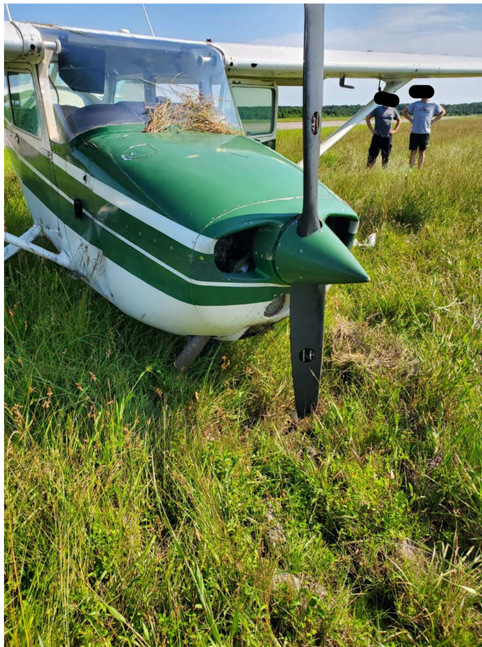
Photo 2 – Right front quarter view of airplane showing substantial damage to fuselage. (Courtesy of Operator)
