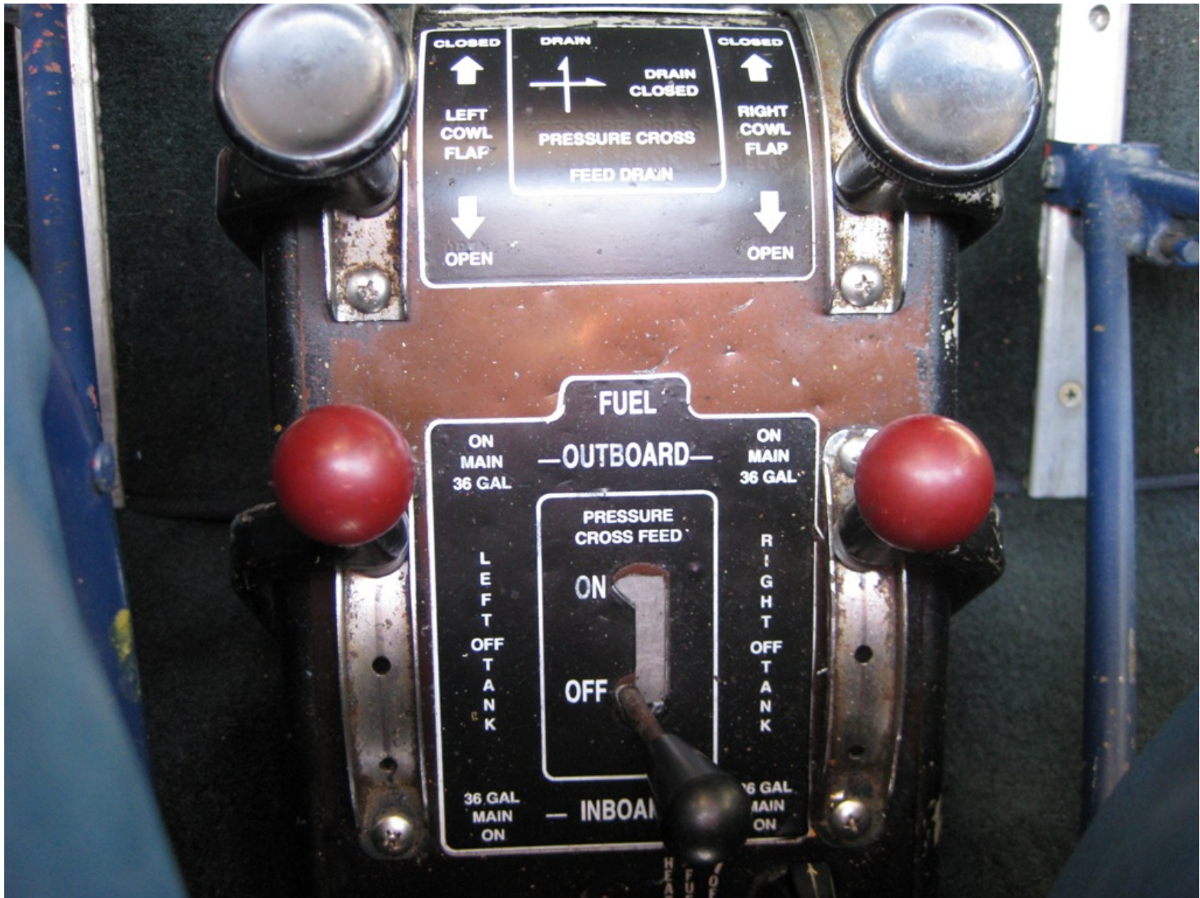
Photo 2 – Fuel Selector Handles (Photo Courtesy of FAA)
