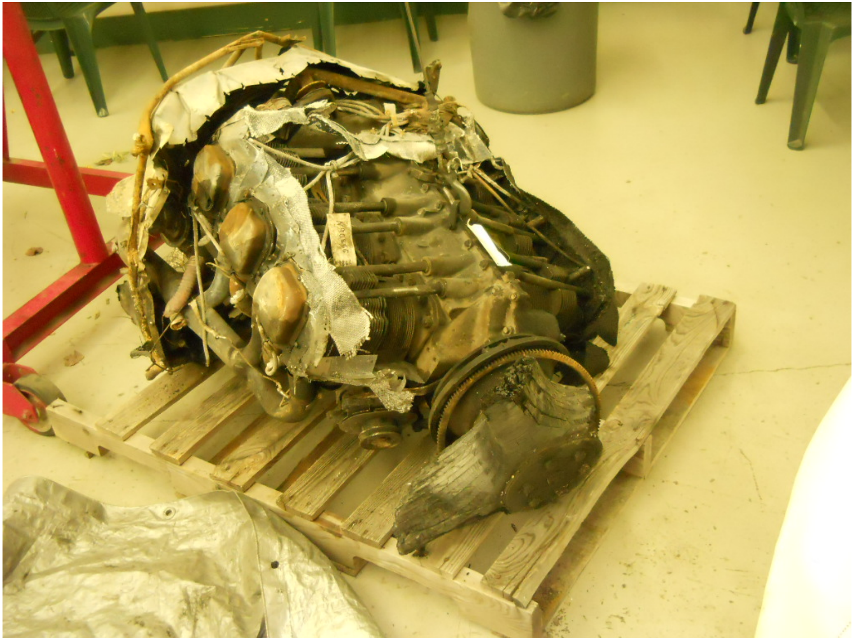
Photo 4 – Engine Recovered
