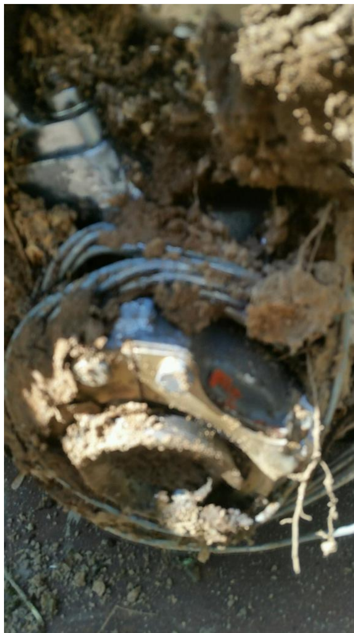
Photo 3 – Engine With Utility Cable Wrapped Around (Photo Courtesy of FAA)
