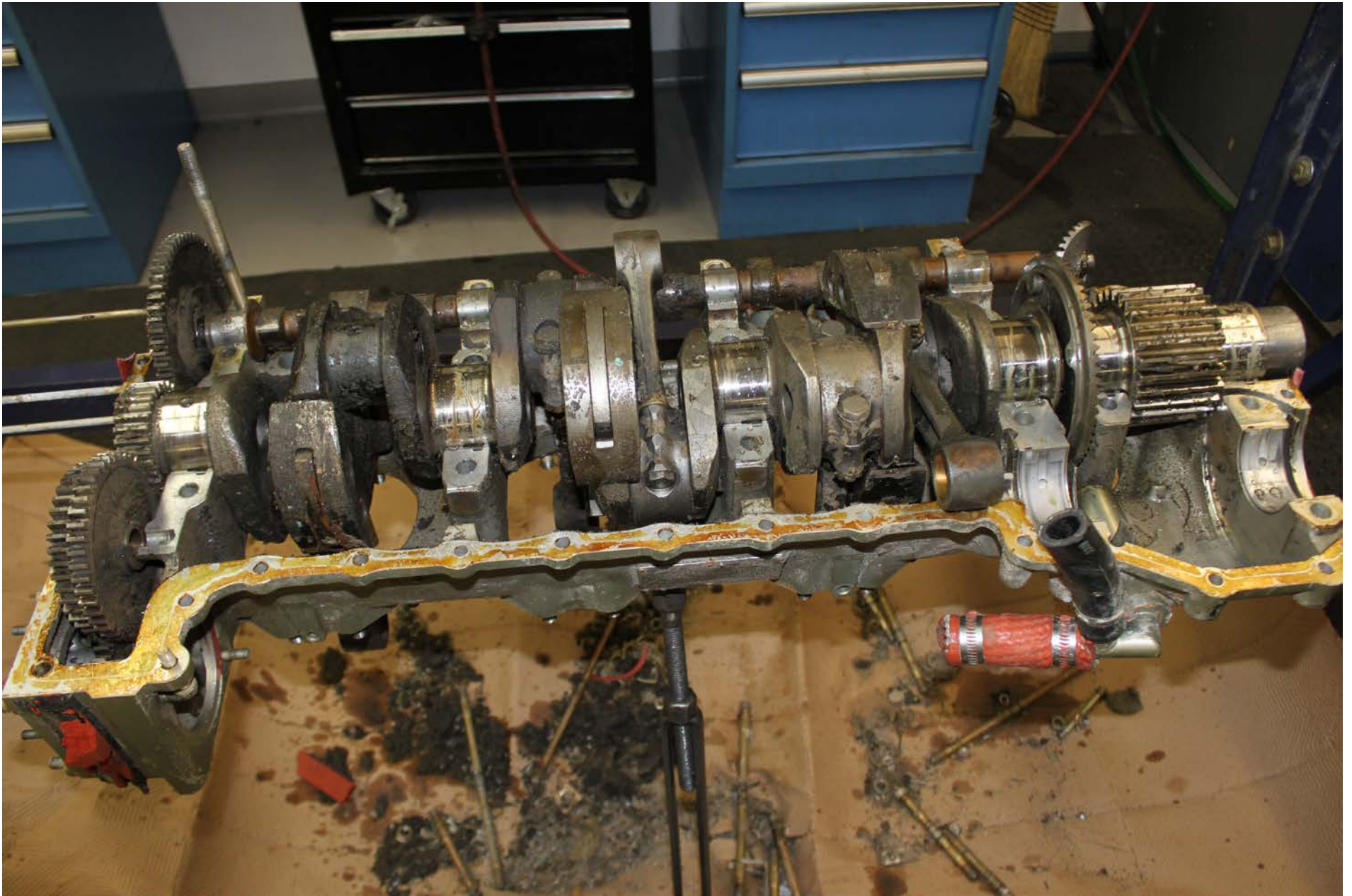
Photo 8 – Left engine during engine examination
