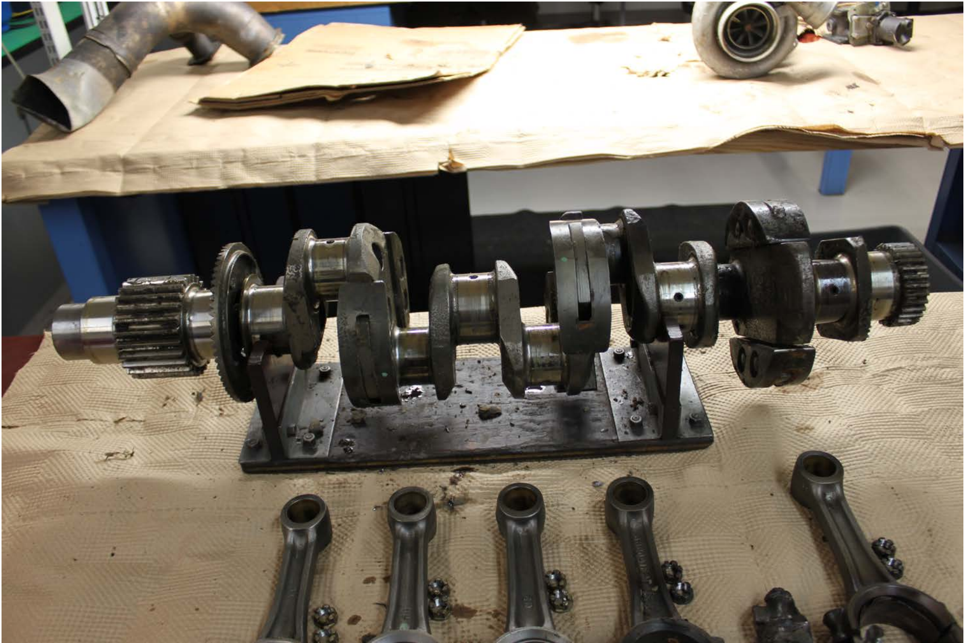
Photo 9 – Left engine crankshaft after removal from engine
