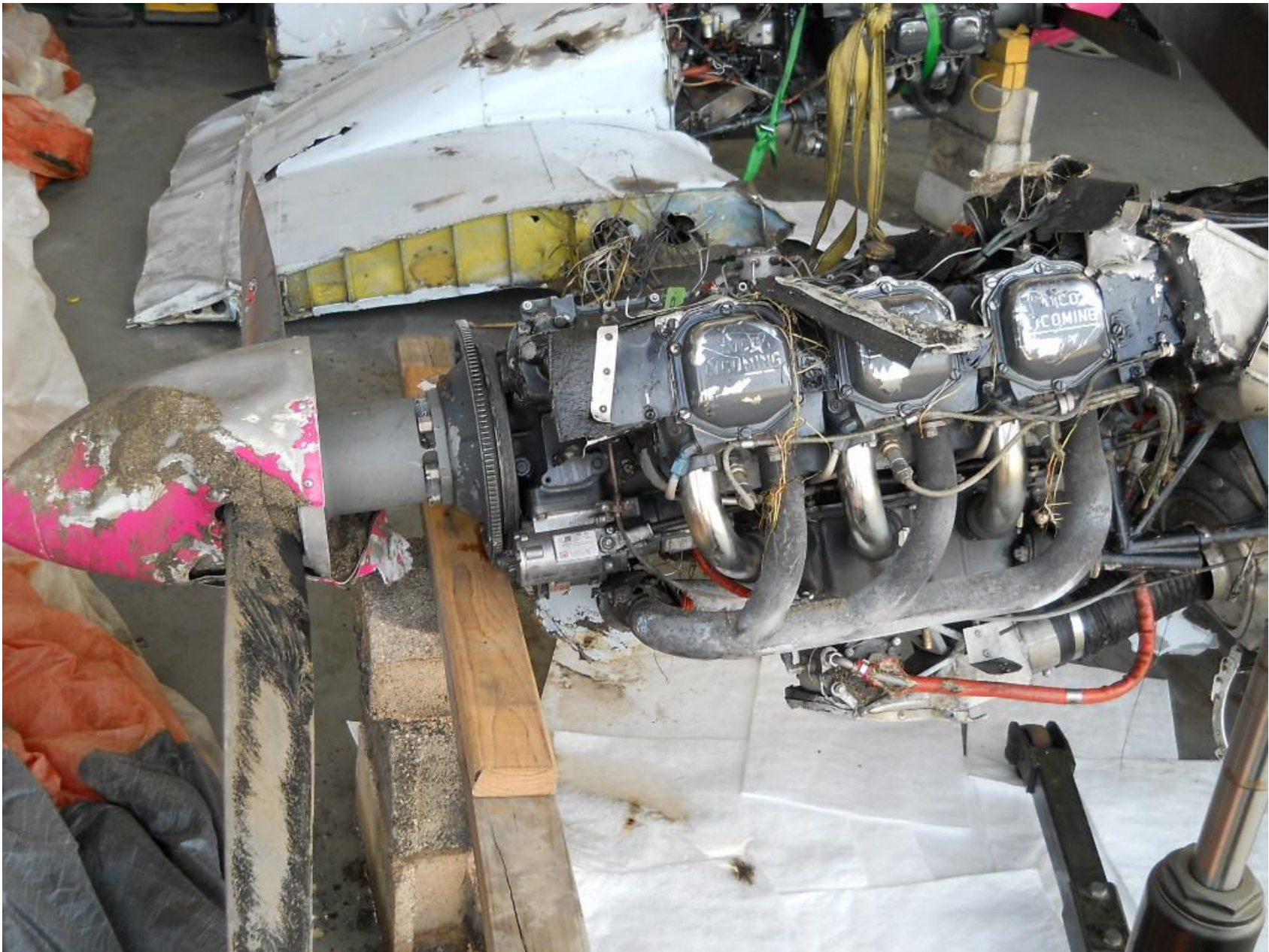
Photo 6 – Right Engine And Propeller
