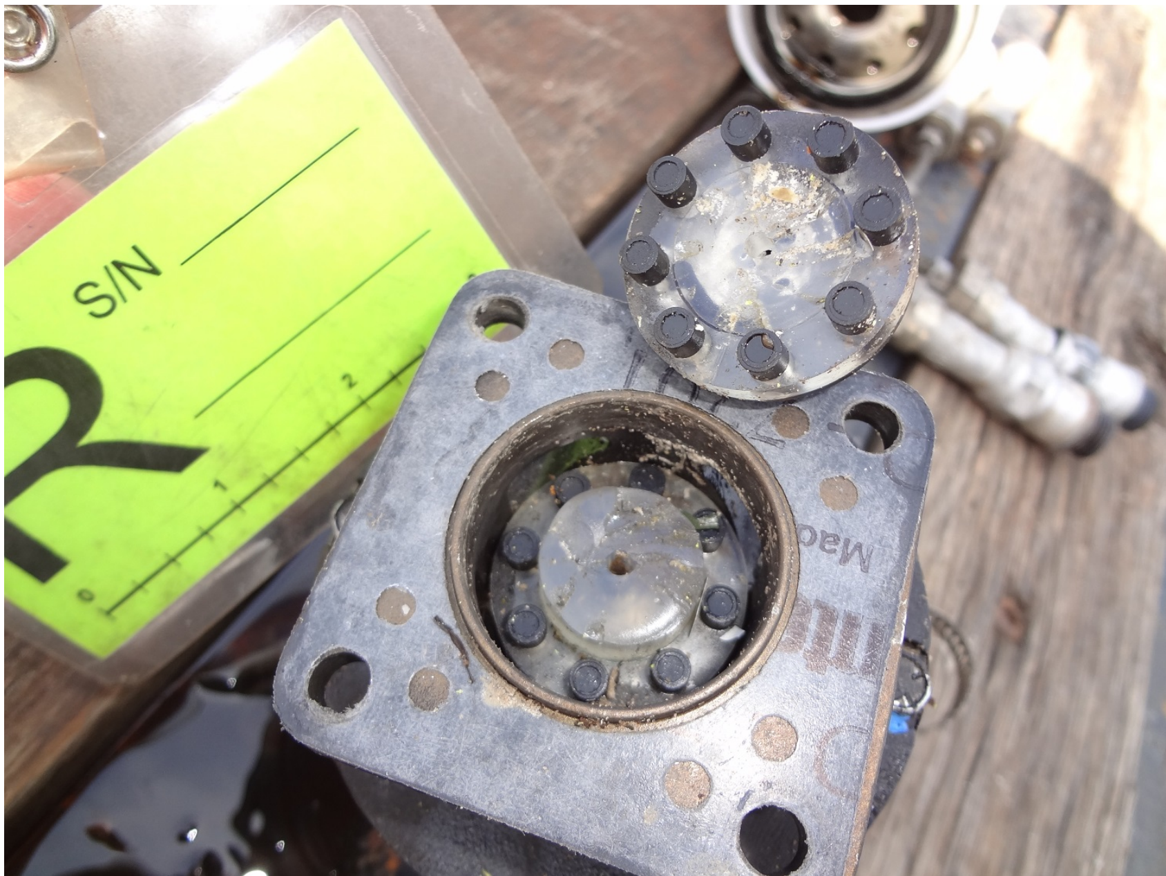
Photo 2 – Right Vacuum Pump as Viewed (Post Recovery)
