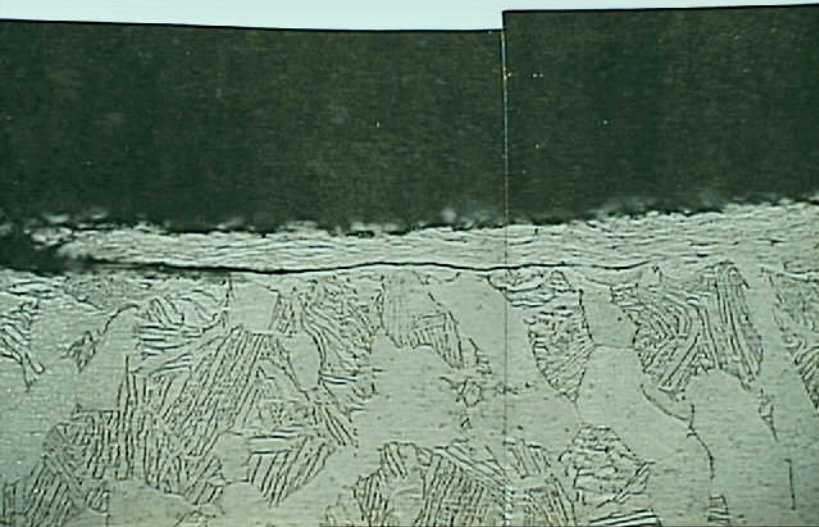
Photo 9. Longitudinal section of hole 2 through a BEA indication, arrow B in photo 7. A chip with deformed microstructure is smeared into the hole surface. Mag.
