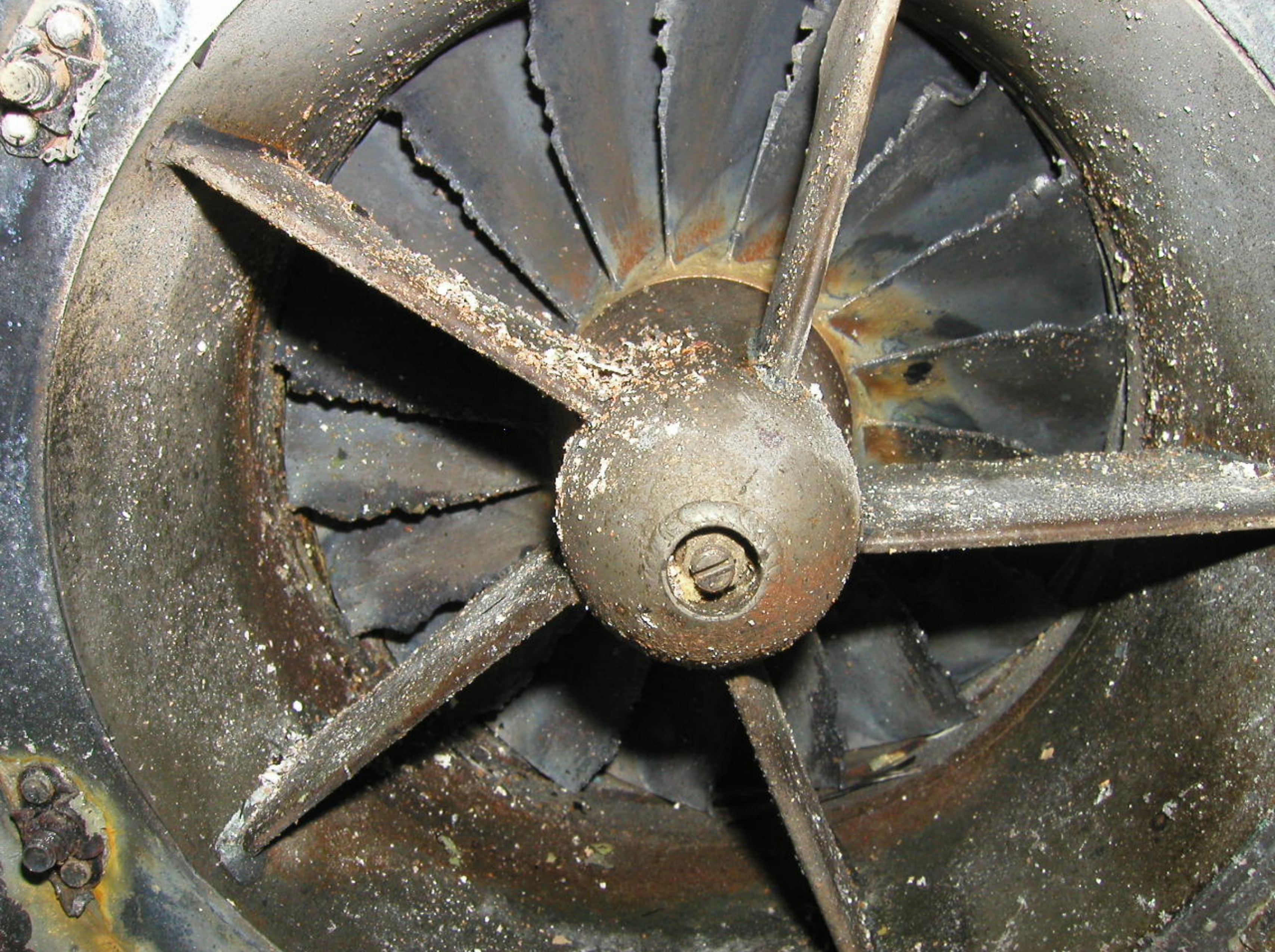
Photo 9. Engine Inlet, Compressor
