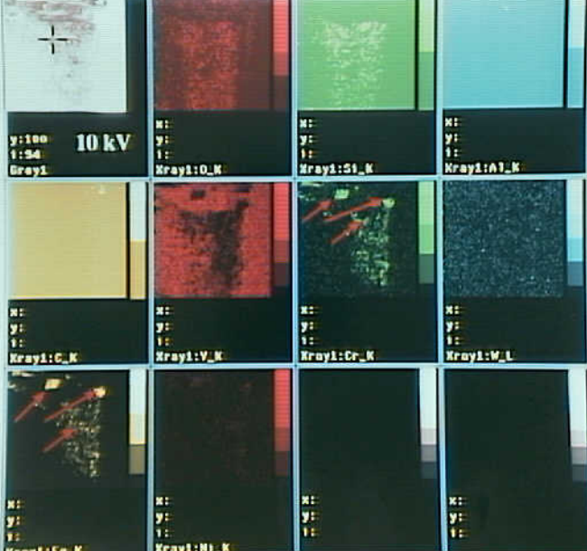
Photo 9. EDS map of Region 5, Figure 8. Elevated concentrations of K-band iron and chromium were identified in the regions of high intensity backscatter electron return (arrows).
