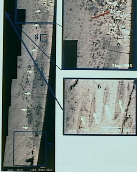
Photo 8. Backscatter electron image of the tierod hole surface. The red arrows identify patches of high intensity electron return. The yellow arrows identify the directional marring. White arrows outline the changed surface morphology near the cracks.
