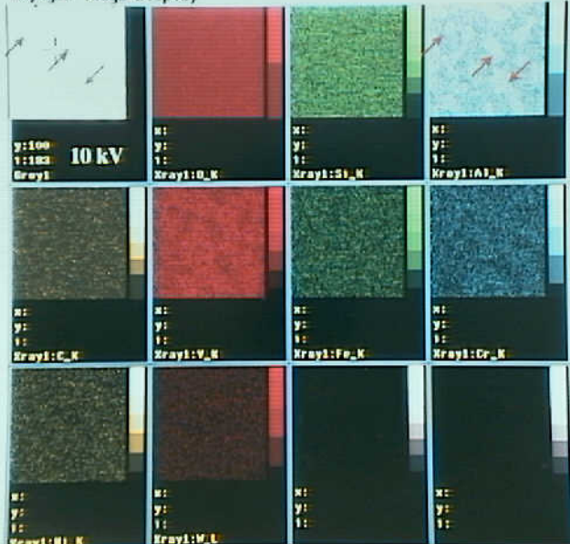
Photo 7. EDS map of bulk microstructure (Region 4, Figure 4.) Elevated concentrations of K-bank aluminum were observed to correspond to equiaxed alpha microstructure (arrows).
