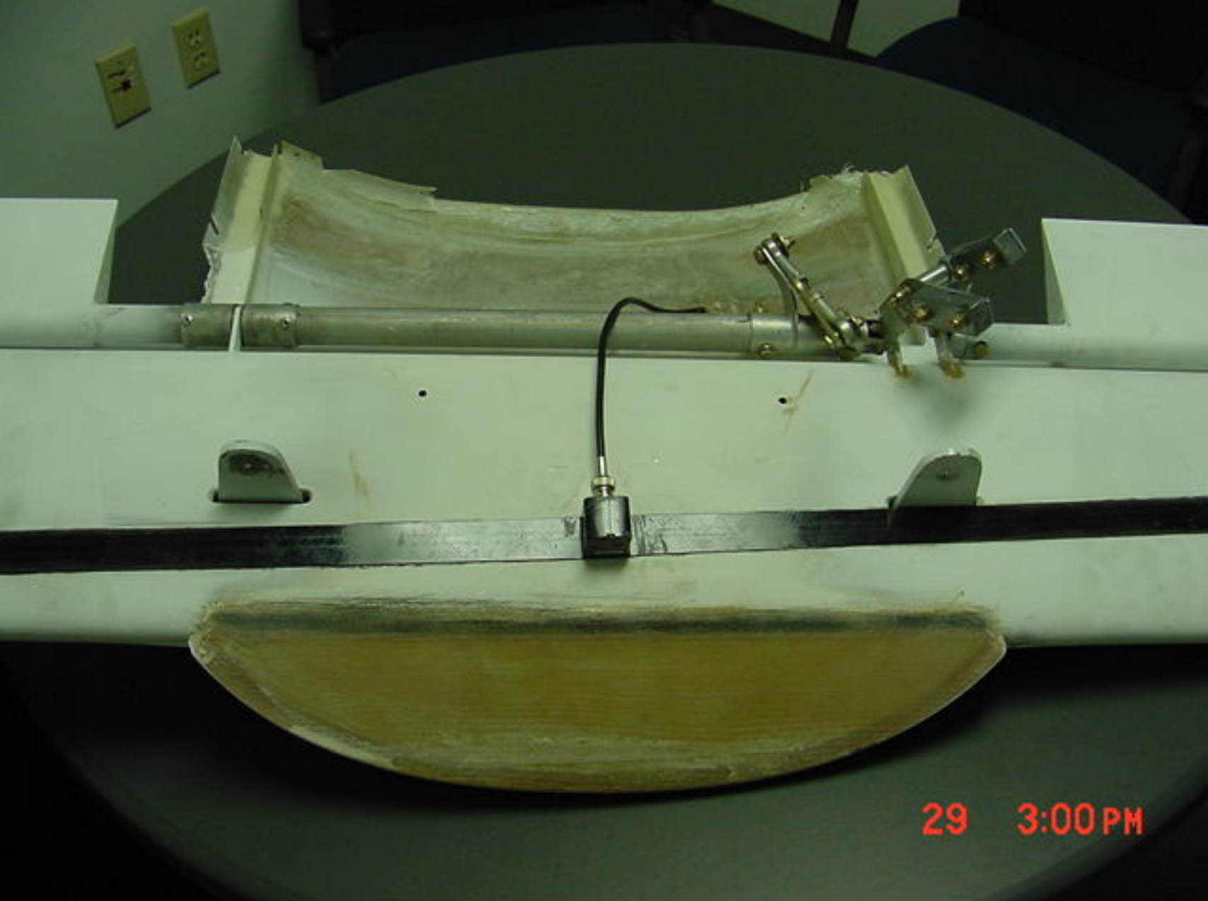
Photo 7. Close-up View of Separated Canard Attachment Hardware
