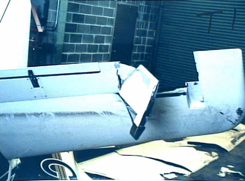
Photo 7. Aft view of right side horizontal stabilizer and elevator.
