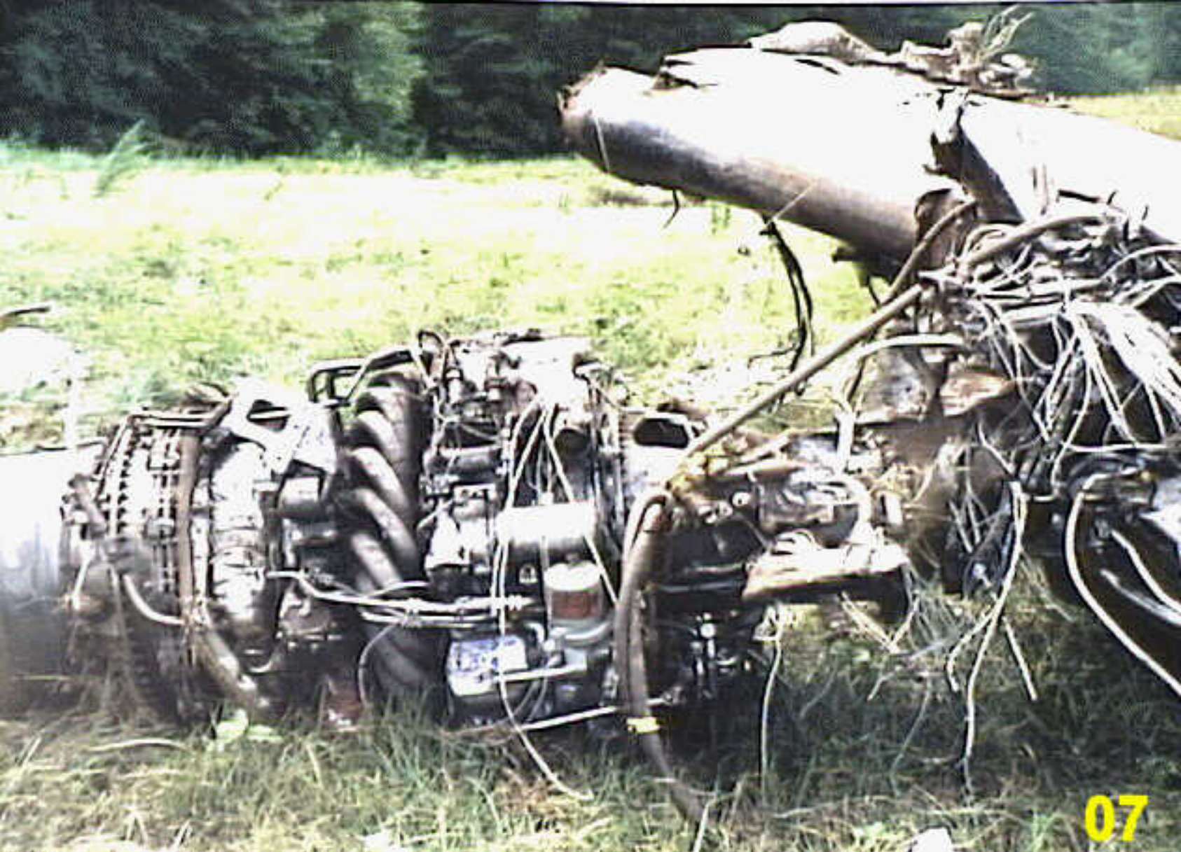
Photo 7 Left Engine and Propeller-Turbomachine at accident site
