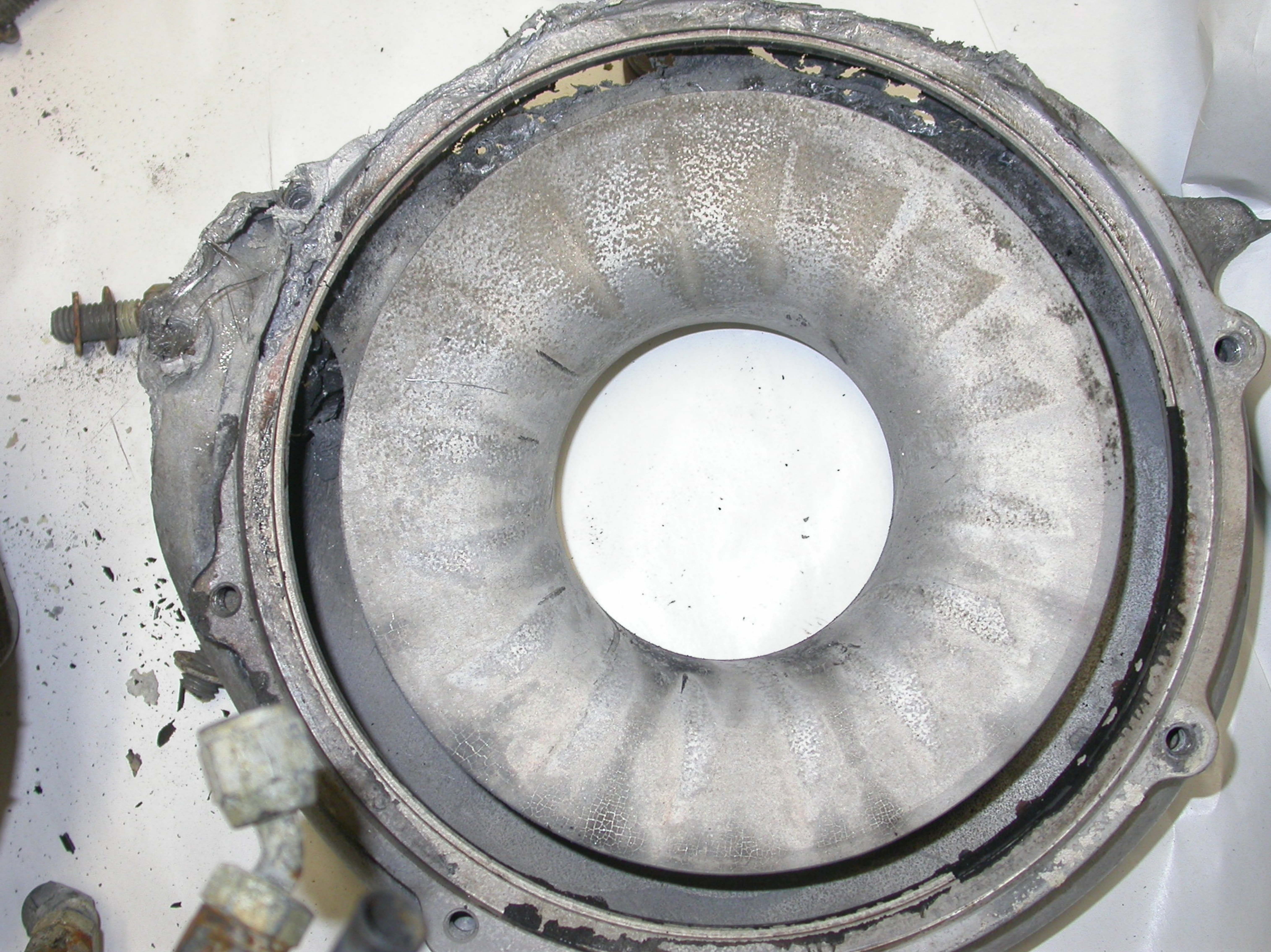
Photo 7: Supercharger Impeller Shroud
