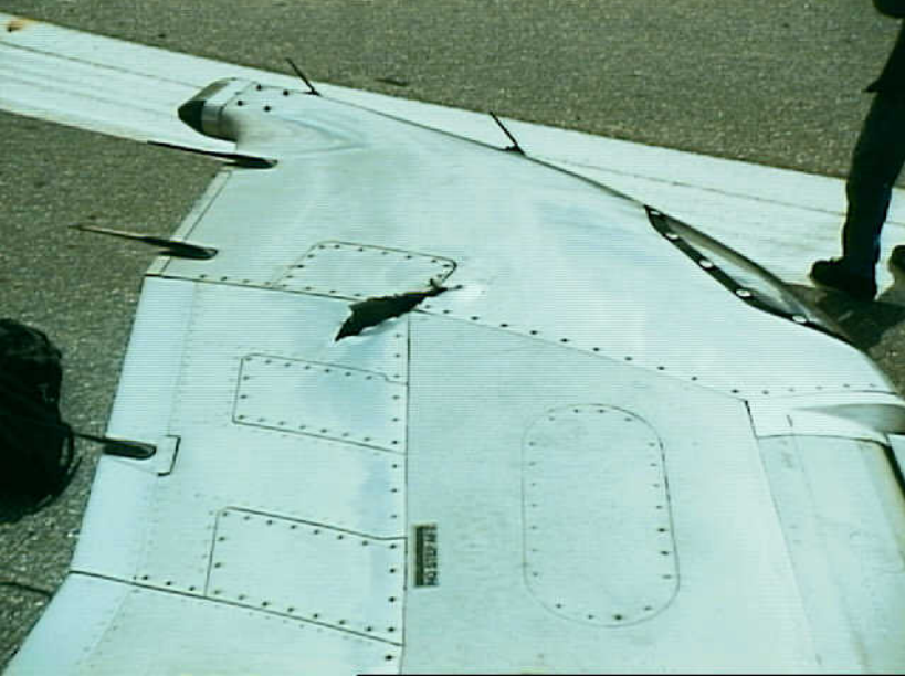
Photo 6. Fragment damage to left wingtip.
