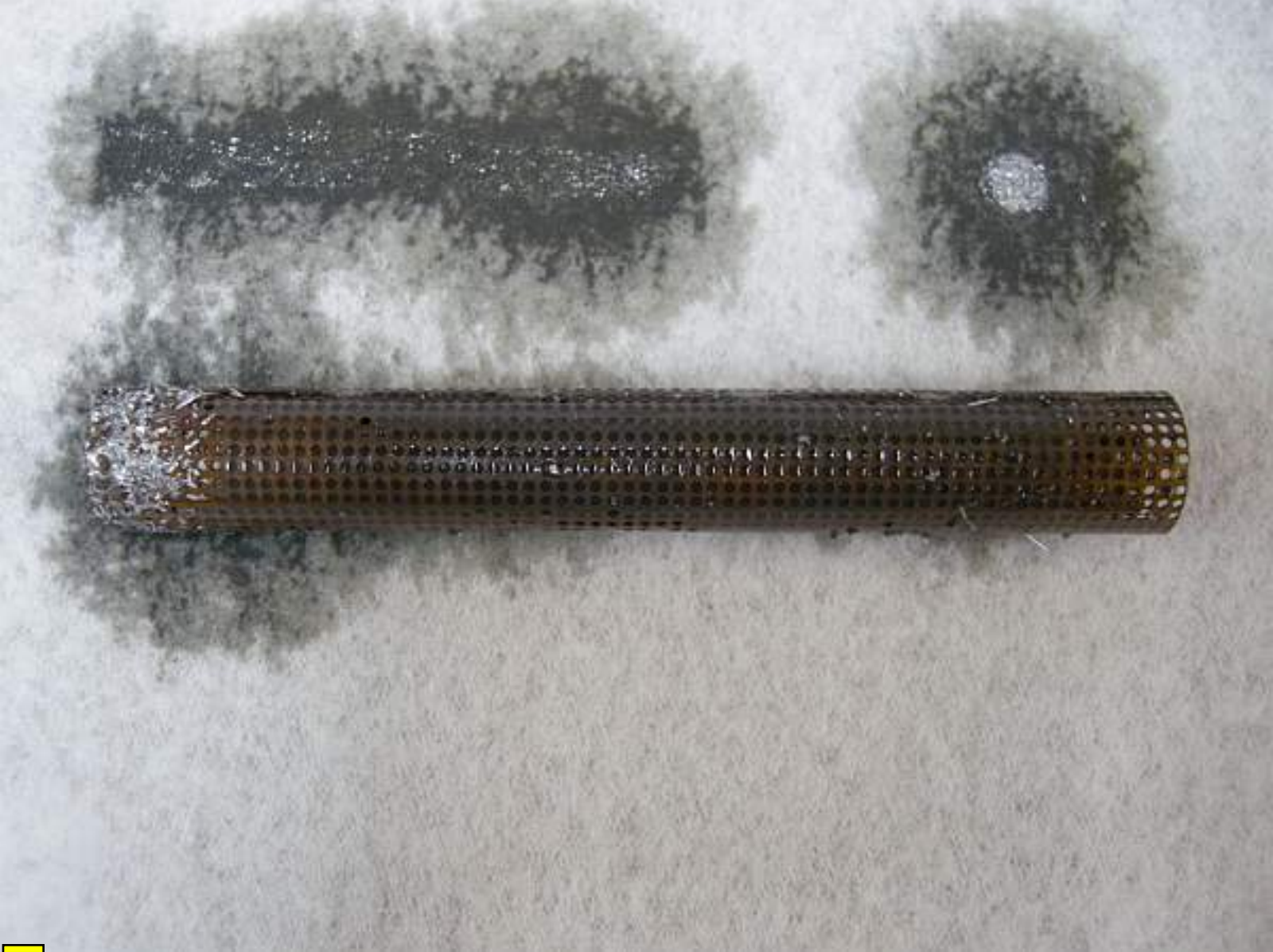
Photo 6 - Aluminum Shavings on Oil Screen
