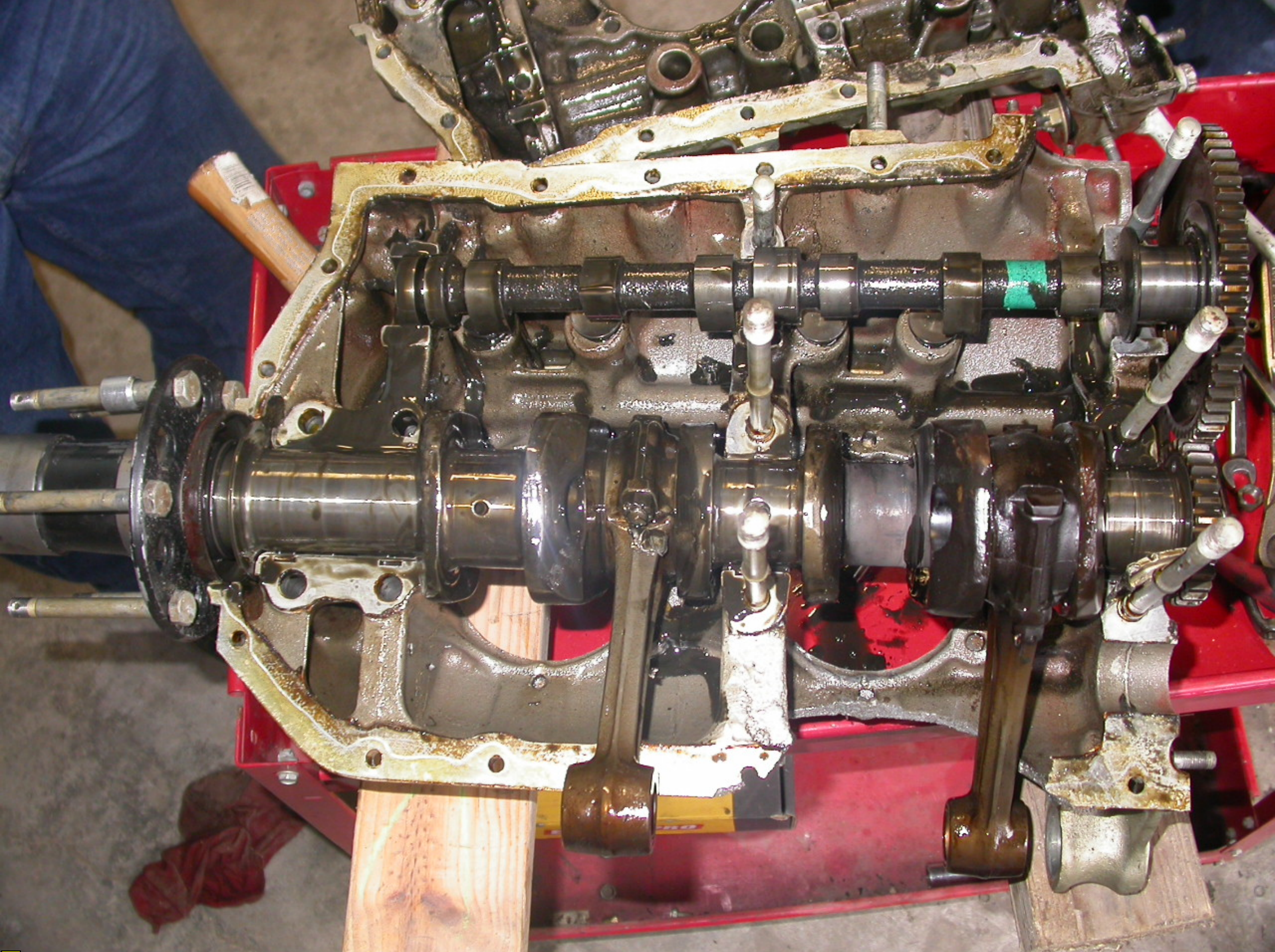
Photo 6: Exposure of the internal engine parts.
