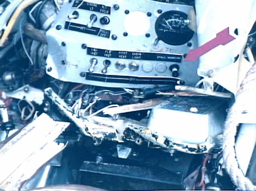
Photo 5. View of Stall warning circuit breaker.
