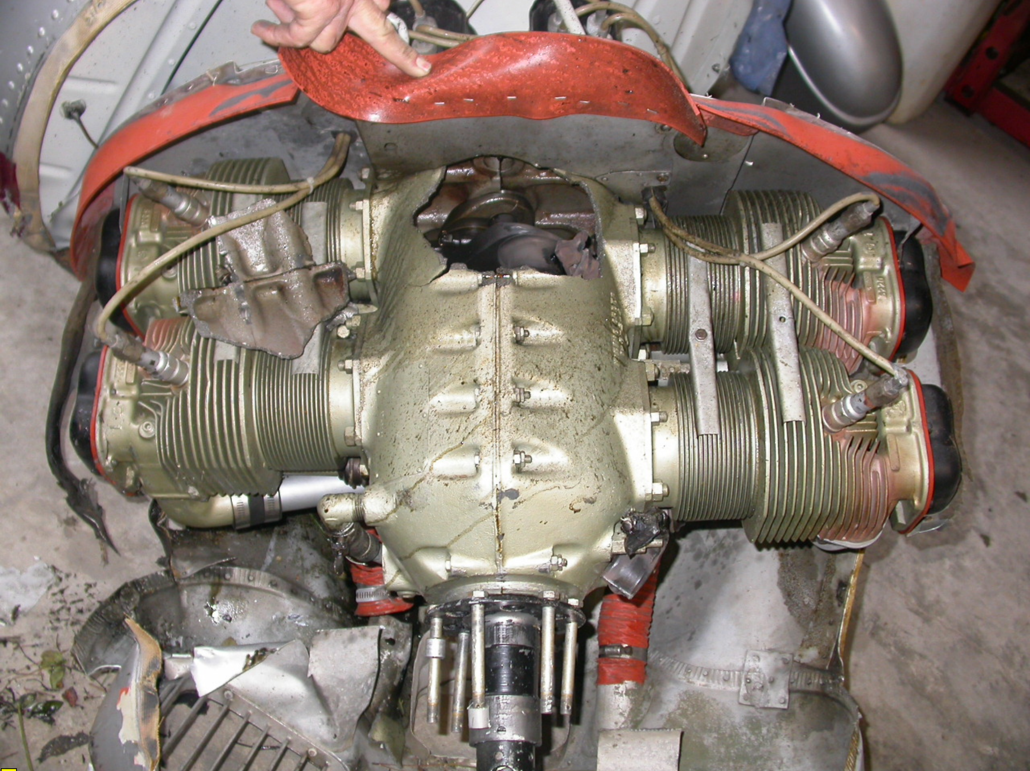
Photo 5: Top side engine damage.
