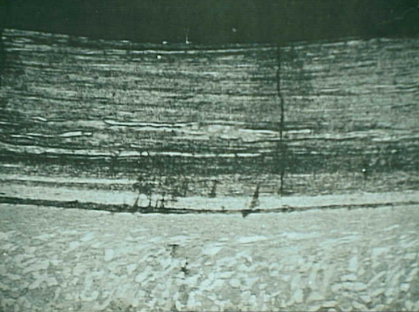
Photo 4. Cross section of hole #2B quite close to the location of the drill breakdown showing a surface layer with cracks and a appearance similar to the failed
