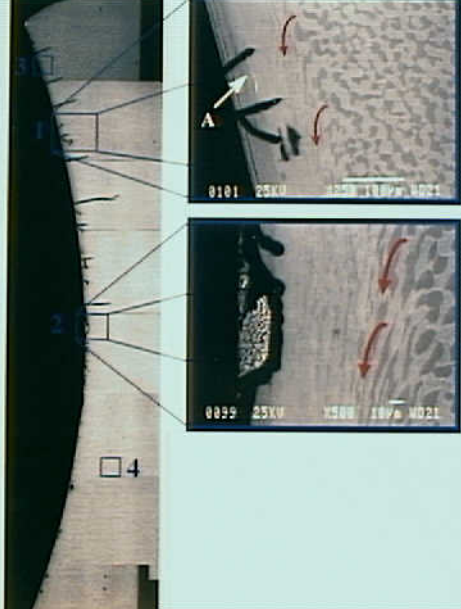
Photo 4. Backscatter electron image photomicrograph of polished surface containing "hardened layer" and at least 29 cracks. The red arrows in Regions 1 and 2 identify observed plastic deformation under the "hardened layer".
