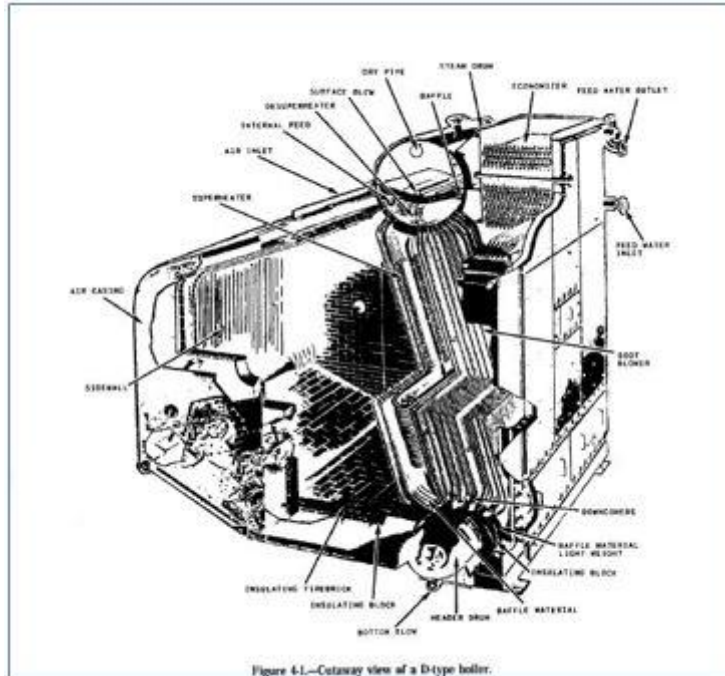
Figure 41.—Cutaway view of a D-type boiler.
