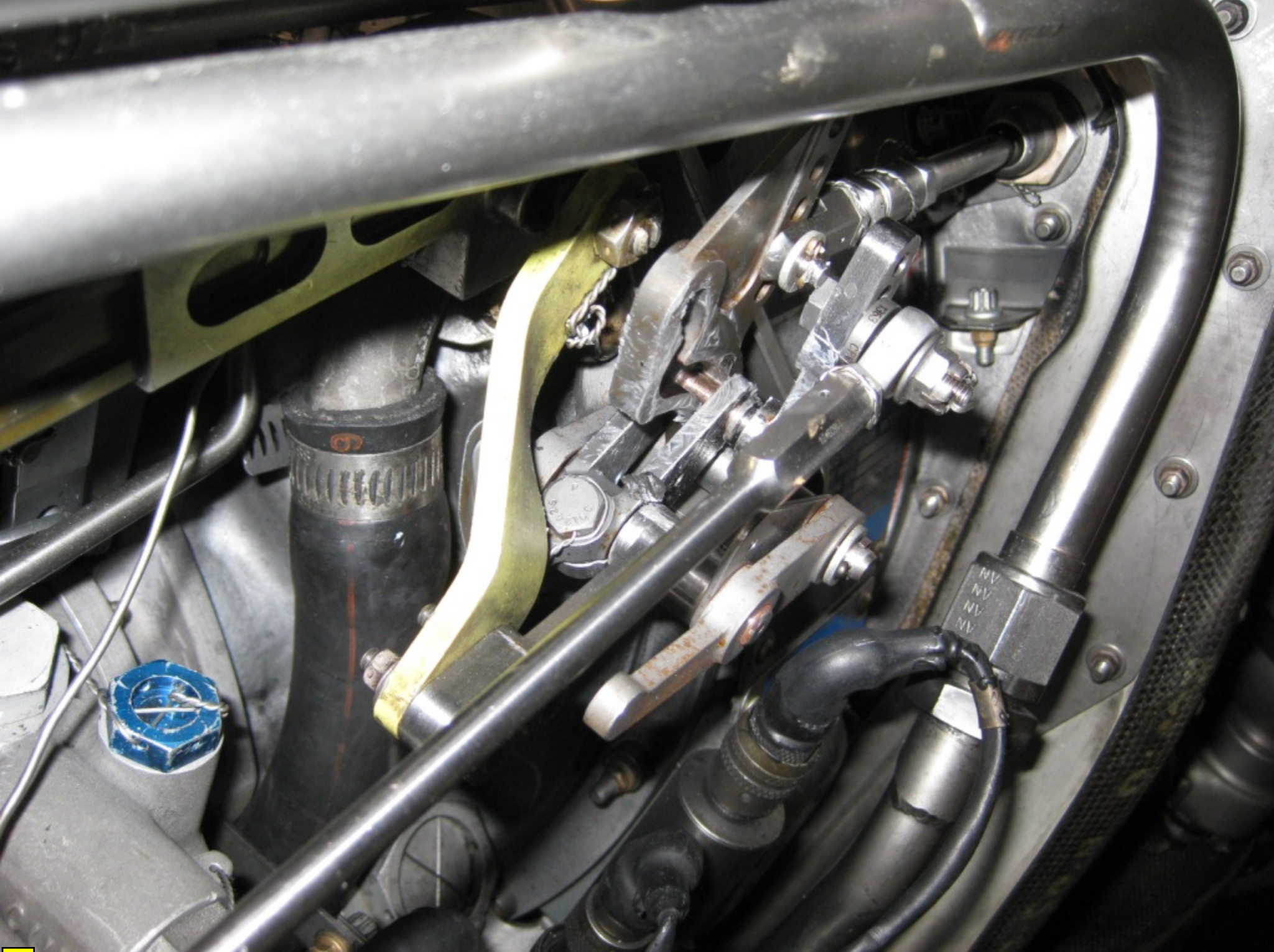
Photo 4 - View of Left Engine Reversing Linkage (FAA)
