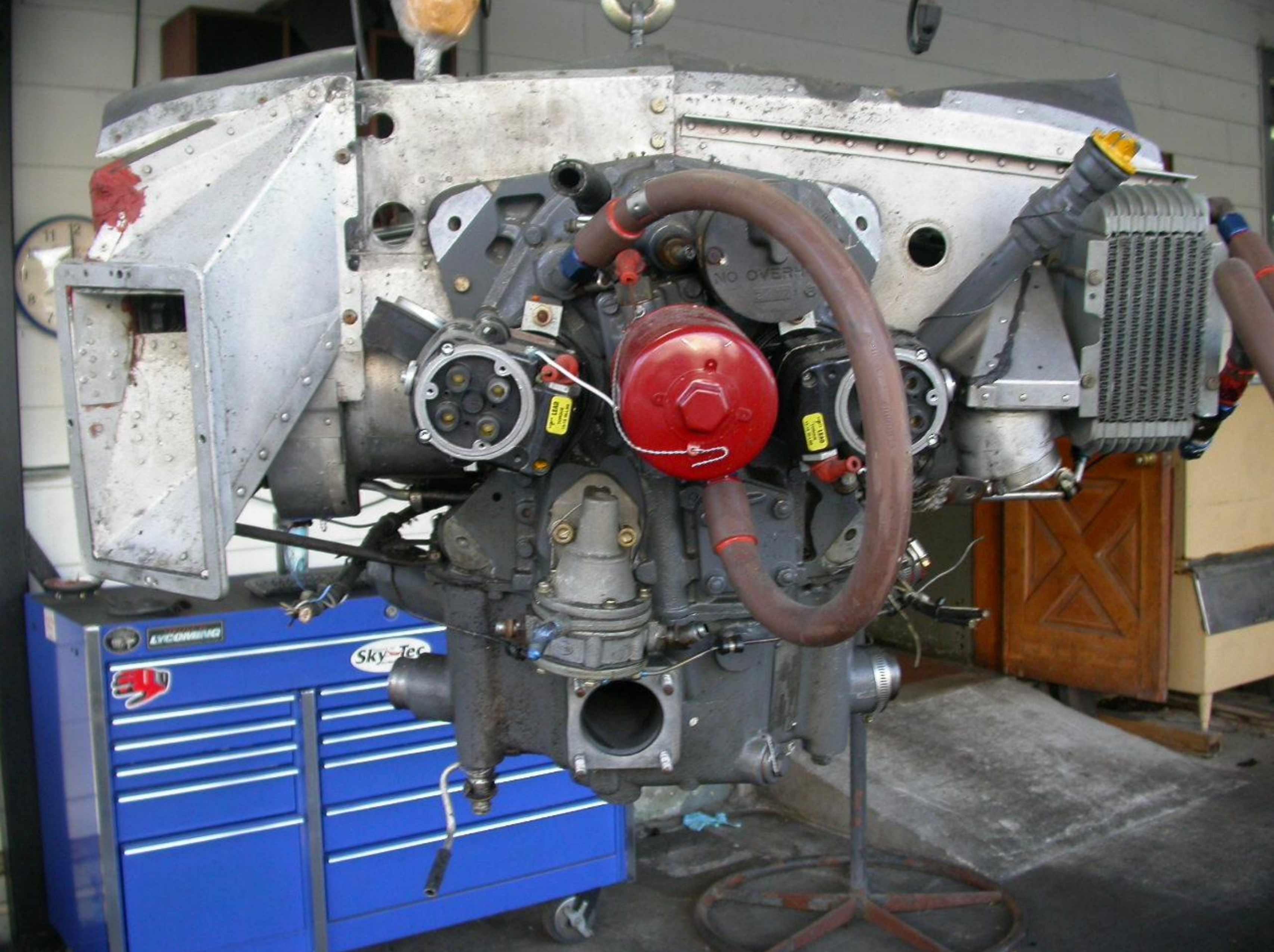
Photo 4) Rear View of Engine.
