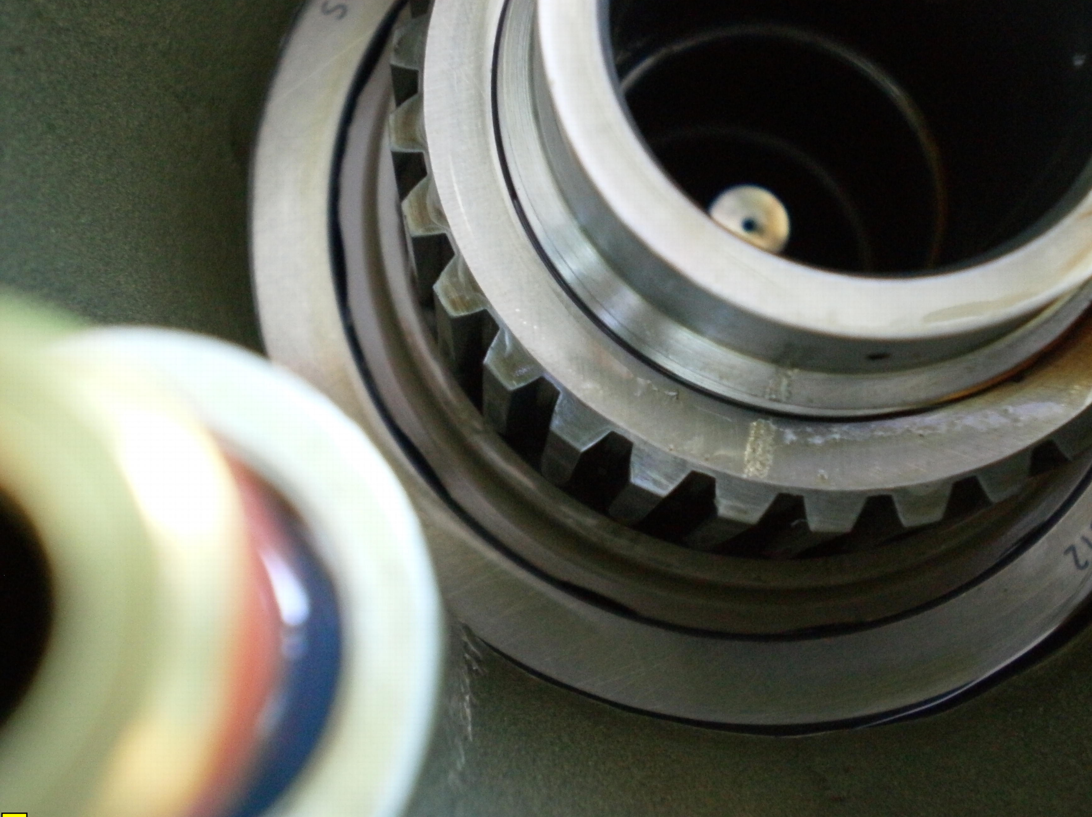
to 37: View of the alignment marks on the input pinion nut
