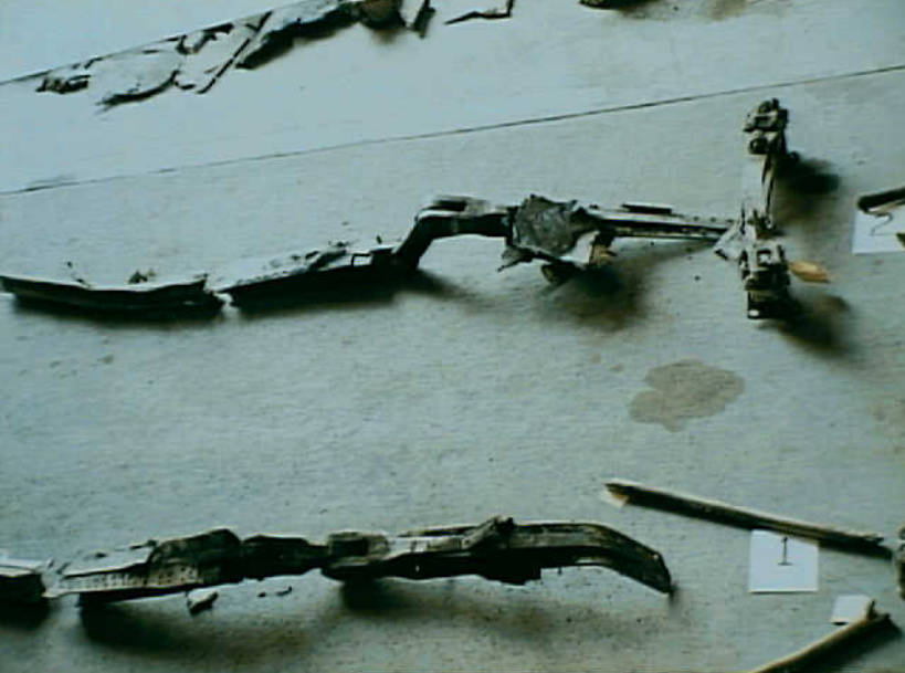
Photo 37. No. 1 & 2 engine and pylon mounts and thrust links.
