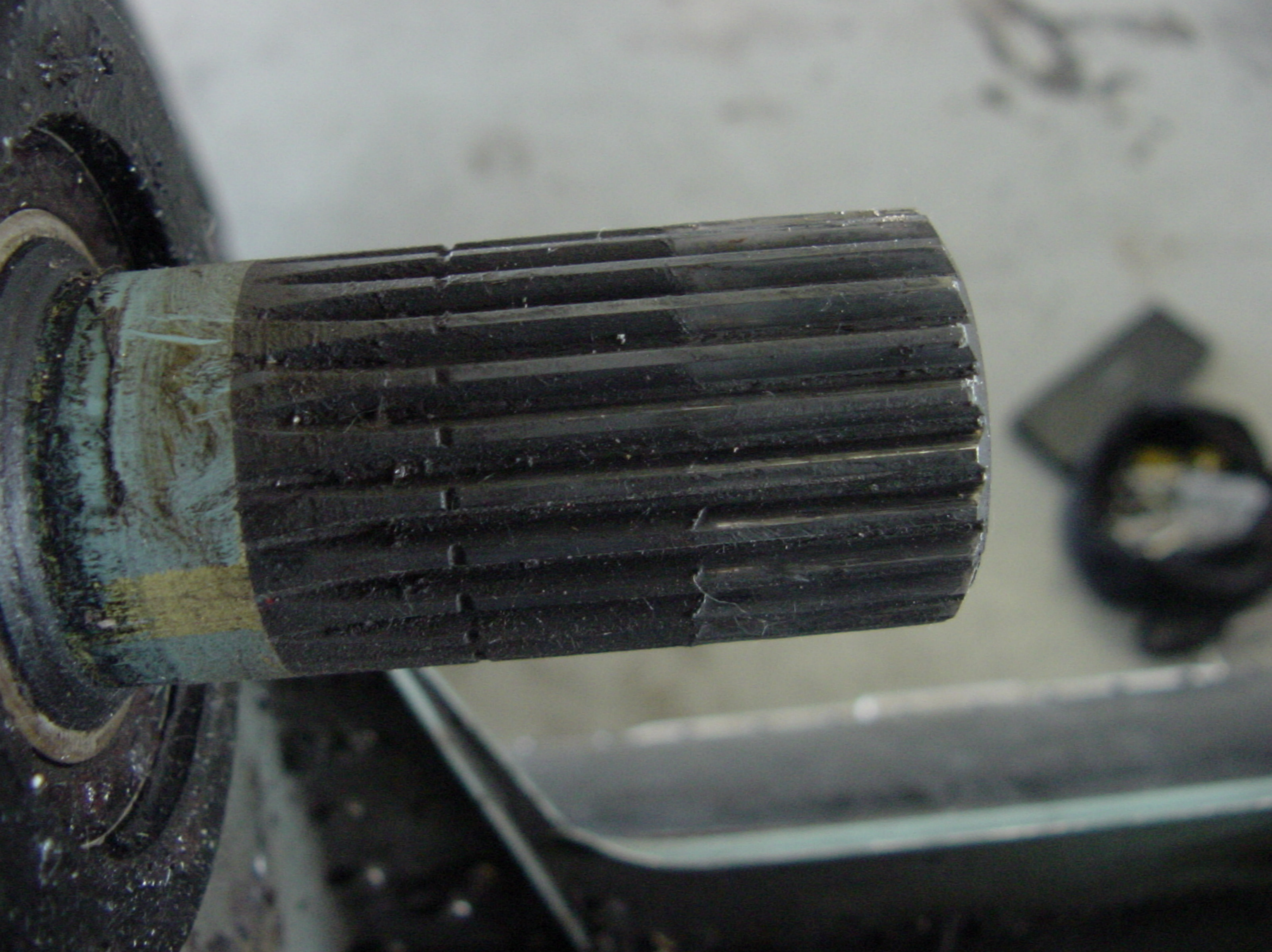
Photo 37. Adapter Gear on Tail Rotor Drive Long Shaft (Eurocopter Photo)
