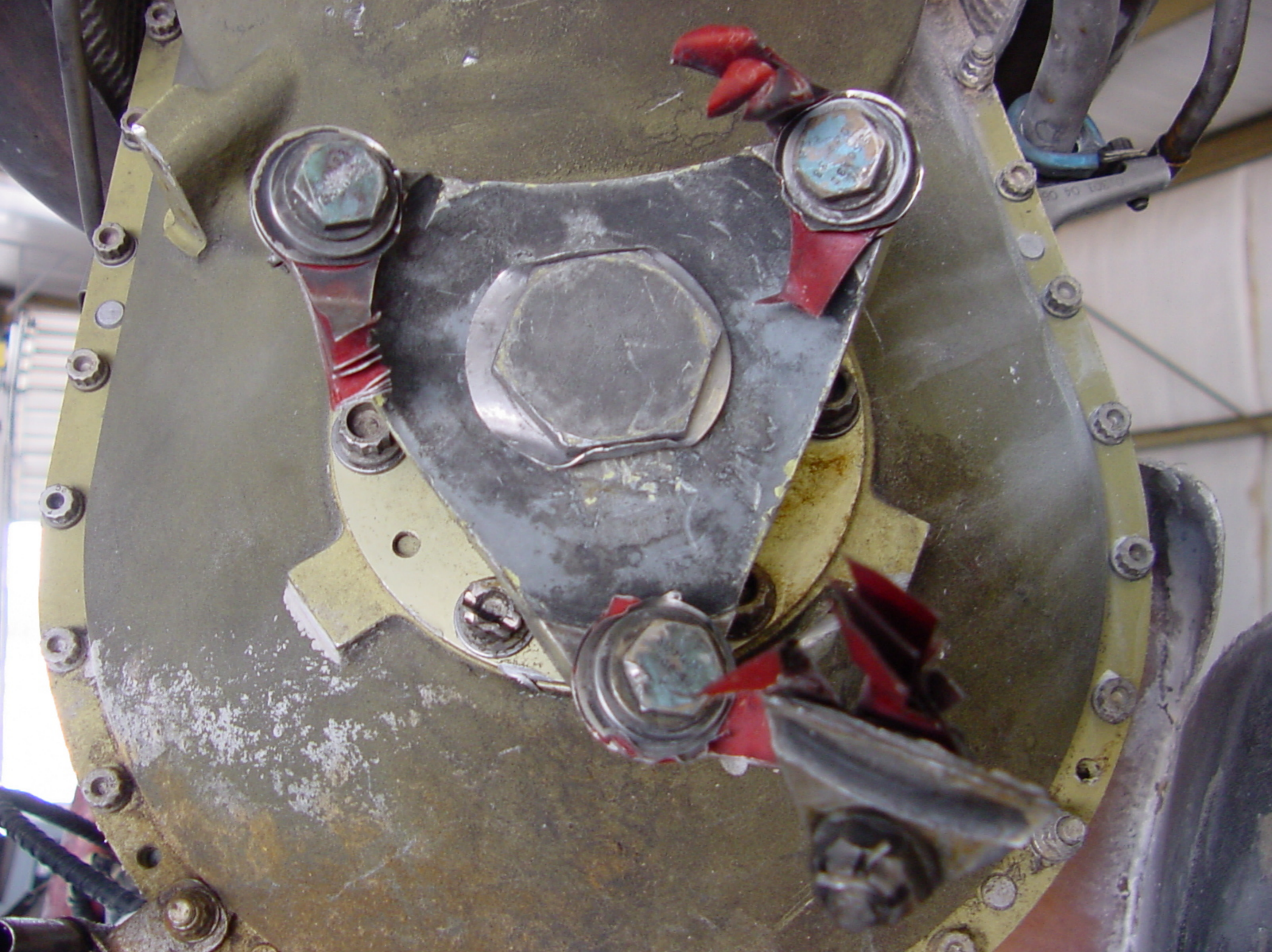
Photo 35. Tail Rotor Drive Flange Coupling (Eurocopter Photo)
