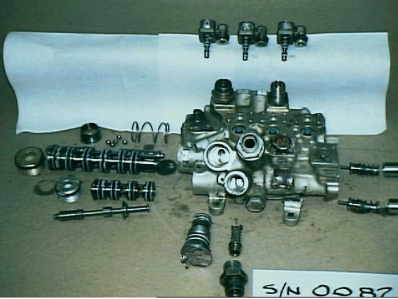
Photo 34. No. 1 engine reverser control valve module
