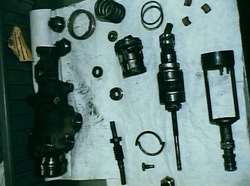
Photo 33. No. 2 engine reverser hydraulic actuator upper outboard locking head.
