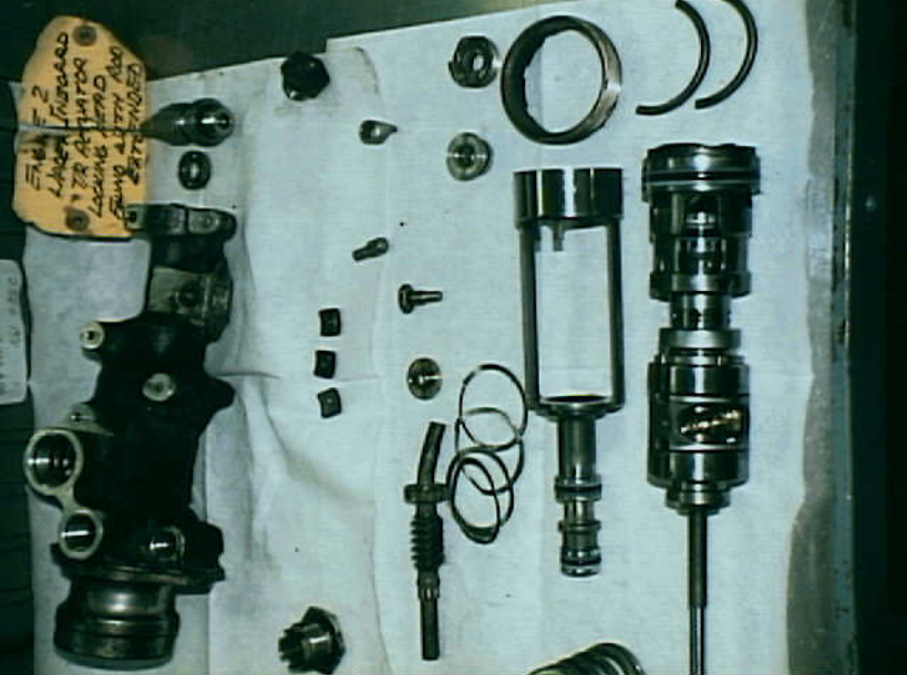
Photo 32. No. 2 engine reverser hydraulic actuator upper inboard locking head
