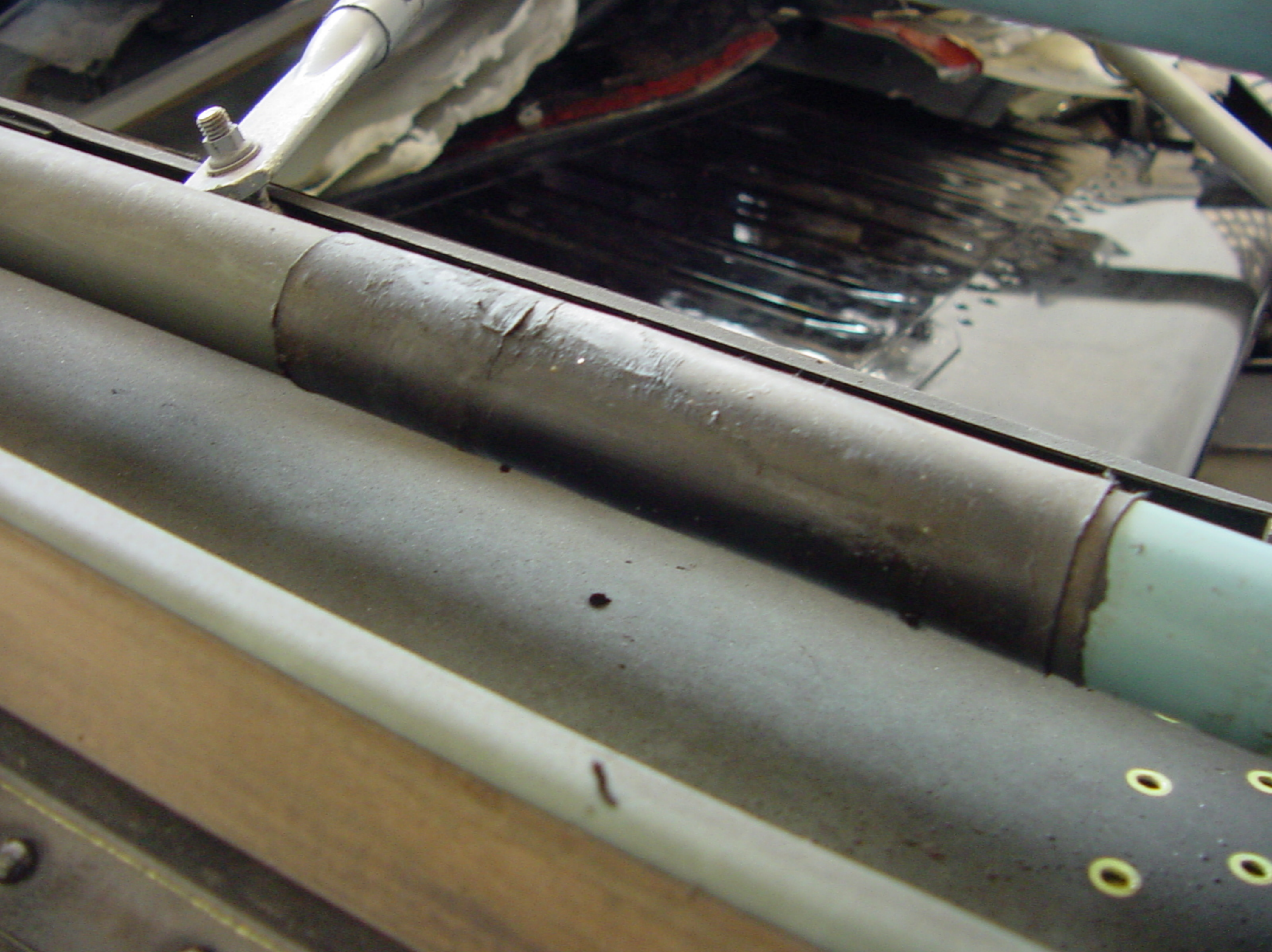
Photo 30. Close-up View of Scuff Sleeve
