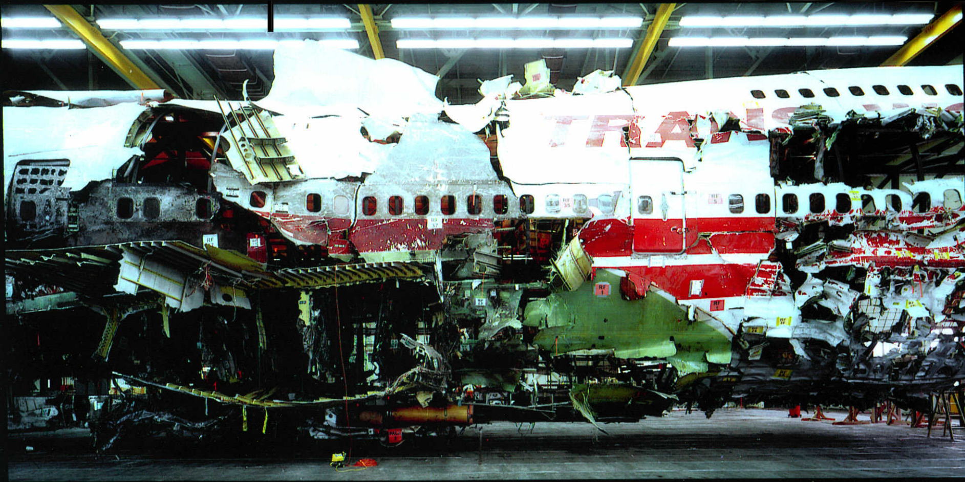
Photo 3. TWA800 - Original fuselage reconstruction
