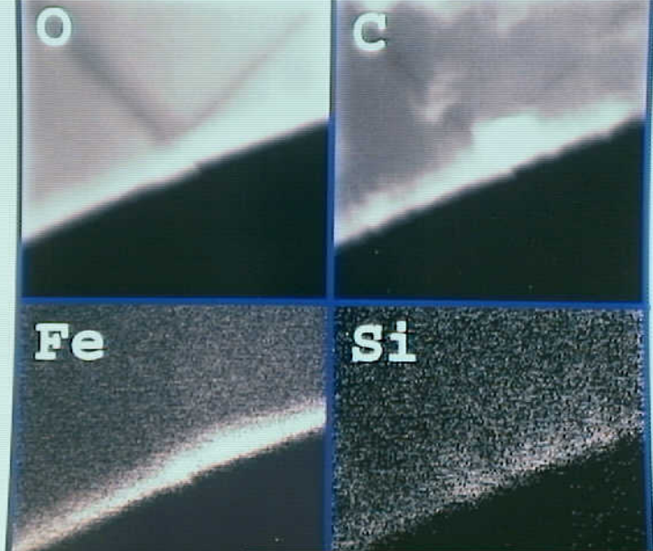
Photo 3. Oxygen, carbon, iron, and silicon SIMS maps of the second region examined. Elevated concentrations (more white) of oxygen, carbon, and iron were observed in the "hardened layer".
