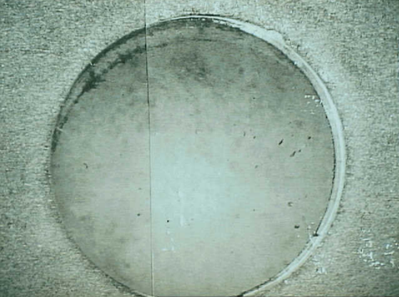
Photo 3. Cross section of hole #2B quite close to the location of the drill breakdown. Mag. 7-8X.
