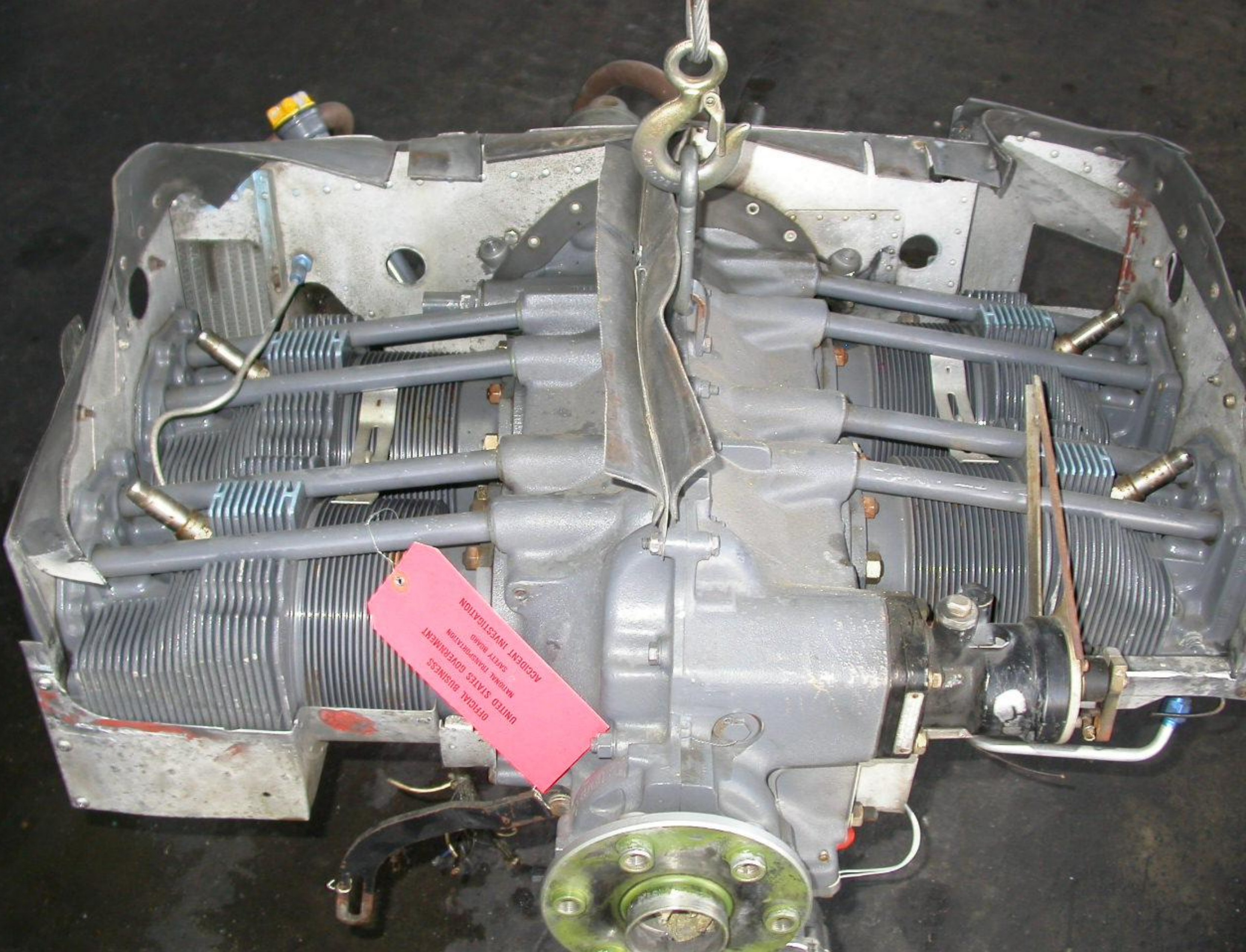
Photo 3) Top View of Engine.
