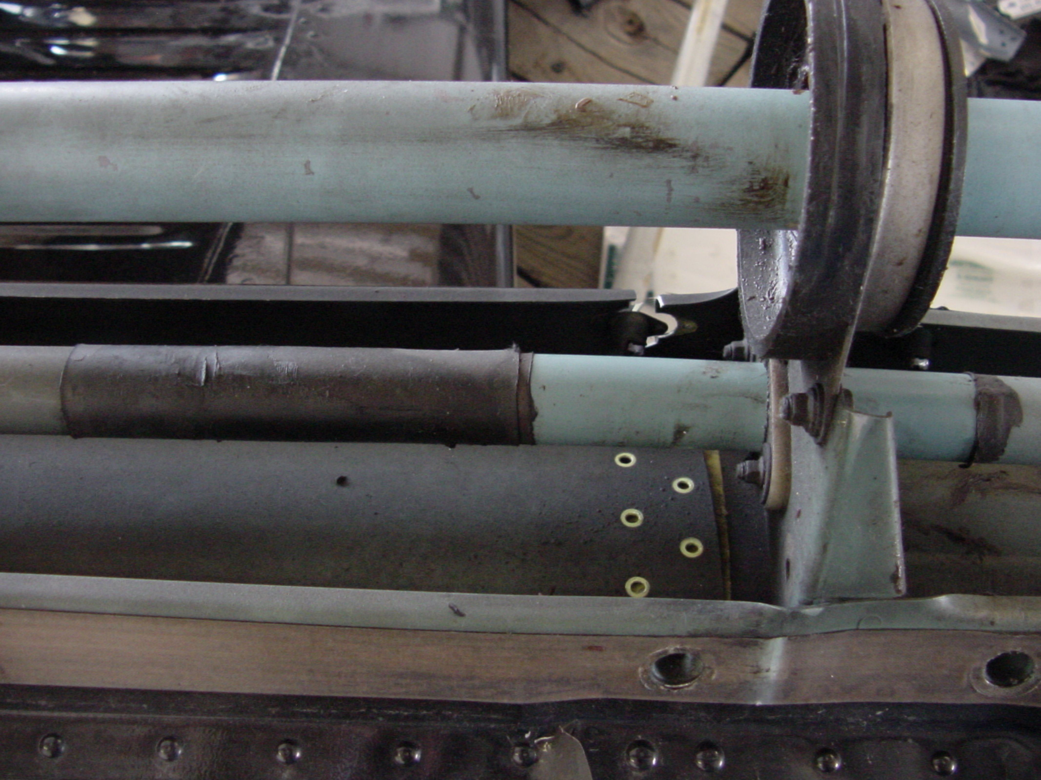
Photo 29. Scuff Sleeve for 4th Bracket (Eurocopter Photo)
