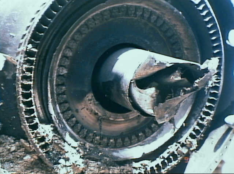
Photo 28. No. 2 engine LPT shaft
