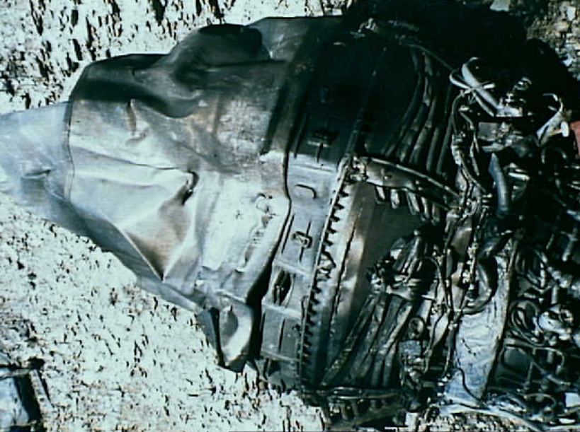
Photo 27. No. 2 engine combustor case, turbine case and exhaust nozzle.
