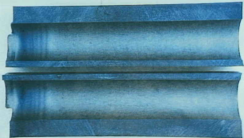
Photo 27. Hole #52 drilled with increased cutting data with HSS to breakage. The hole has also been fine bored and honed. The hole was blue etched before and after being sectioned into two halves.
