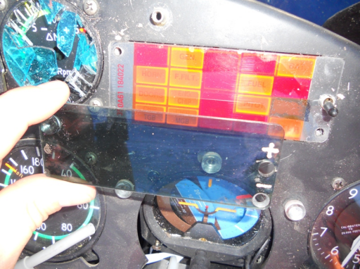
Photo 26: View of caution-warning annunciator panel with NVG lens removed
