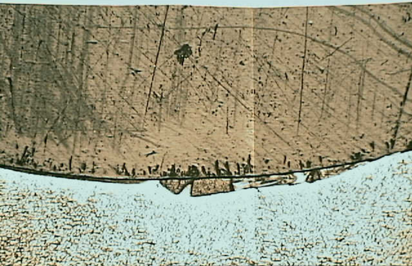
Photo 24. Cross section of the indication area in hole #57. The microstructure shows deformation to a depth of 0.2 mm (0.0079 inch). Mag. 32X.
