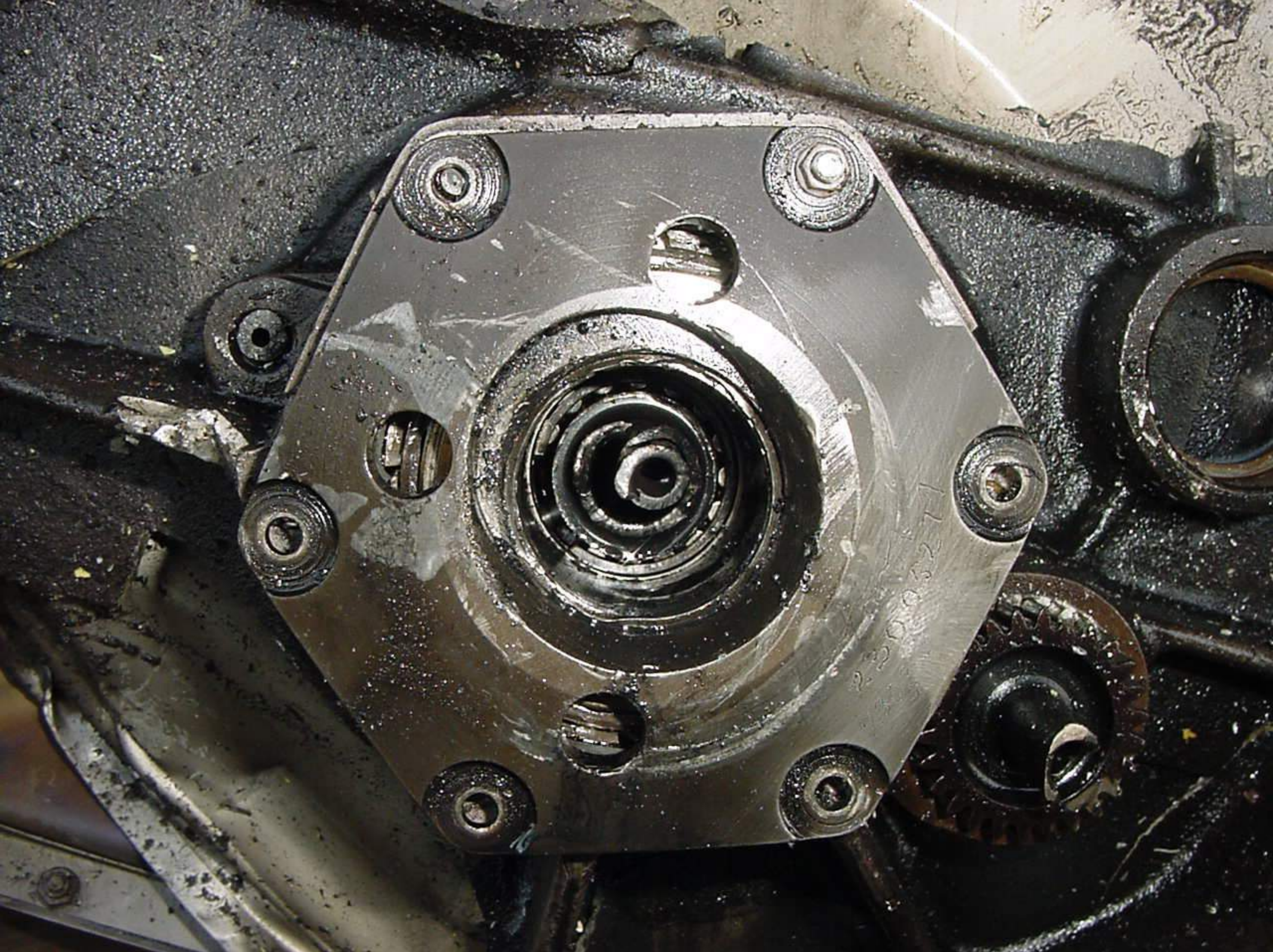
Photo 21. Spur Gearshaft Fracture Overview
