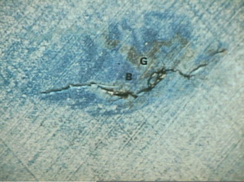
Photo 21. A close up of the center of the BEA indication in hole #1B. The grey area G is contaminated with iron (Fe) in difference with the blue area B. Notice the crack in the area.
